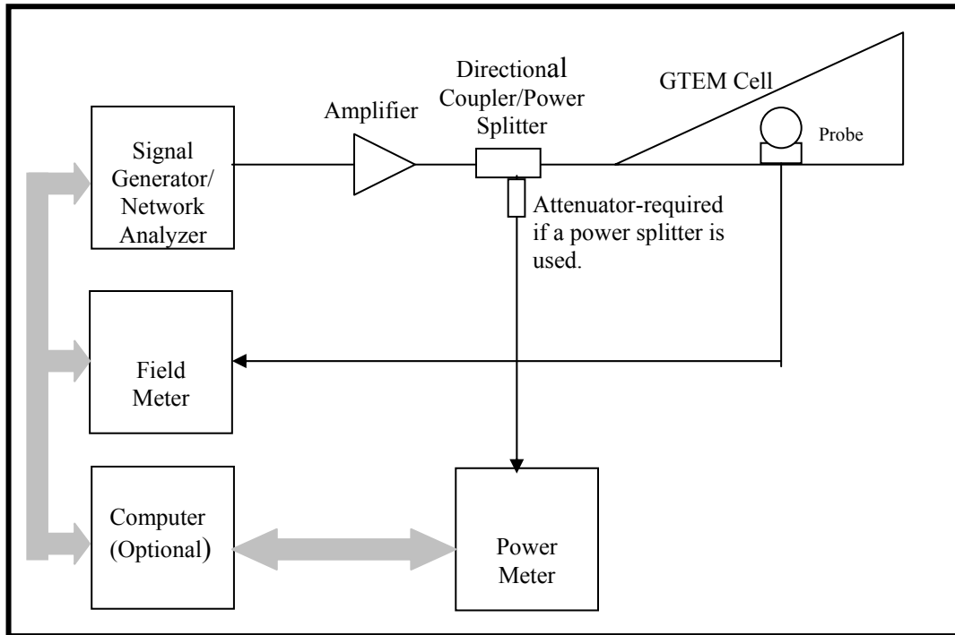
Figure C.1 Field Uniformity Verification Configuration
