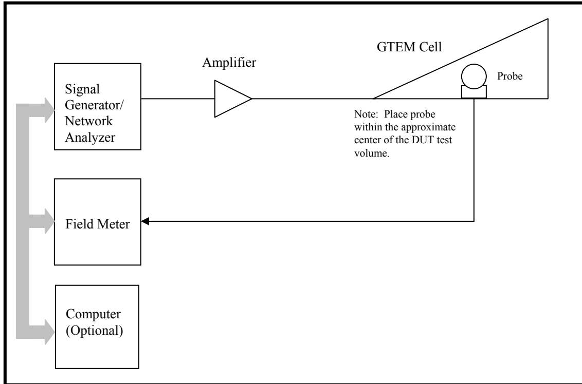
Figure B.1: GTEM Qualification Test Configuration
