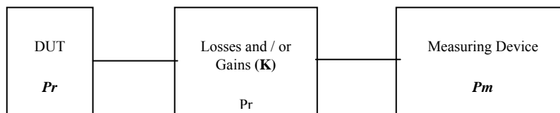
Figure A.1: Receive Path block diagram
