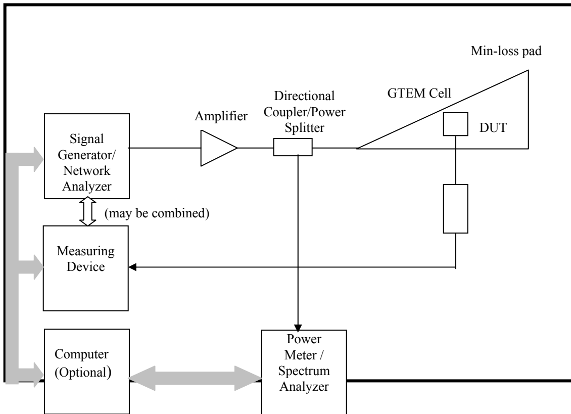
Figure 1: Equipment Setup for Ingress Shielding Test (Method 2)
