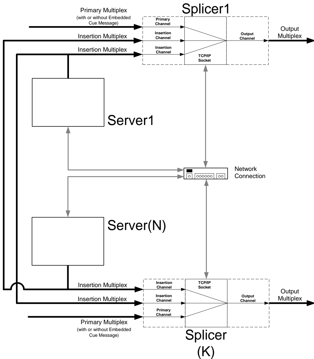
Figure 6-2 Multiple Servers / Multiple Splicers
