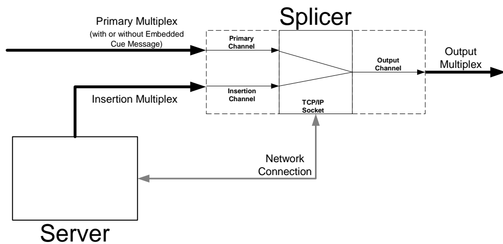
Figure 6-1 Single Server / Single Splicer
