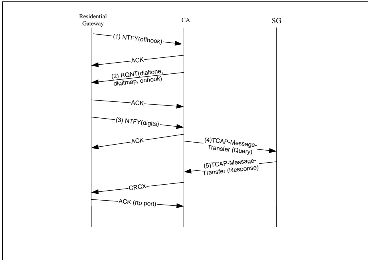
Figure 12. 800 Number Service
