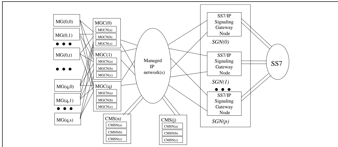
Figure 5. Architecture Model of a Fully Distributed IPCablecom Gateway Employing n+k Redundancy
