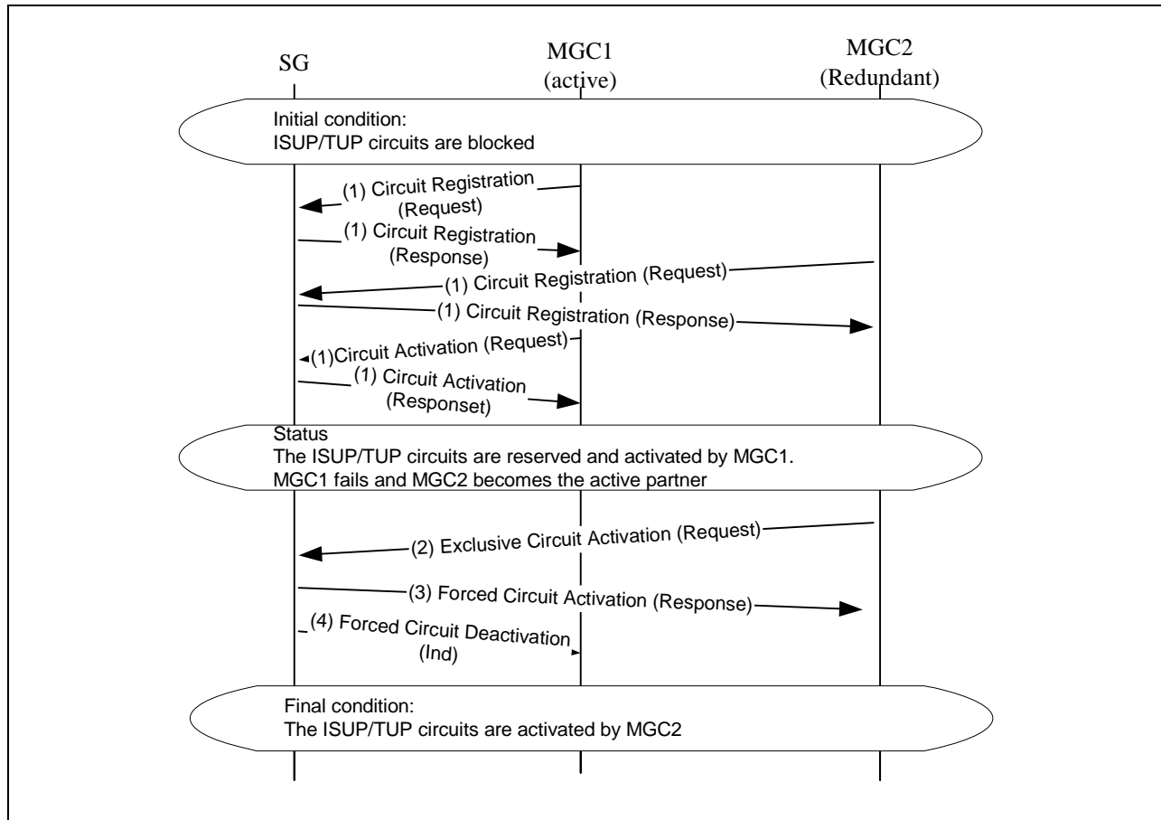
Figure 13. MGC Failover Procedure
