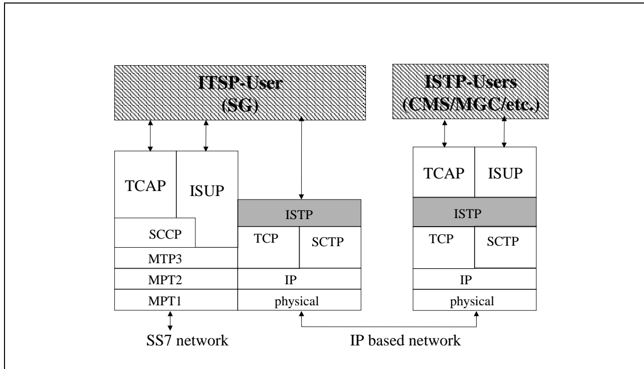
Figure 3. Protocol Distribution in IPCablecom Elements
