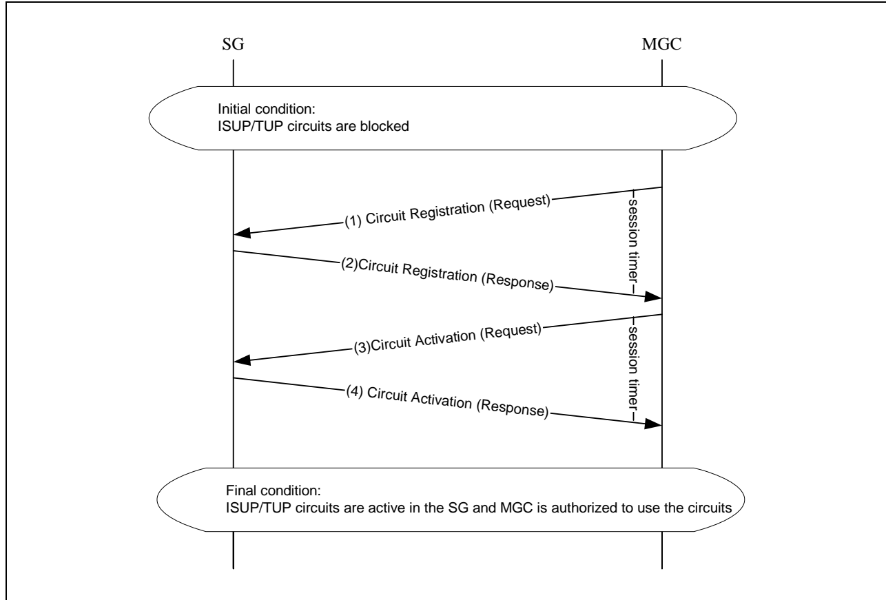
Figure 7. MGC Requests ISUP/TUP Service
