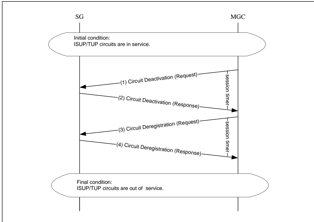
Figure 8. MGC Terminates ISUP/TUP Service
