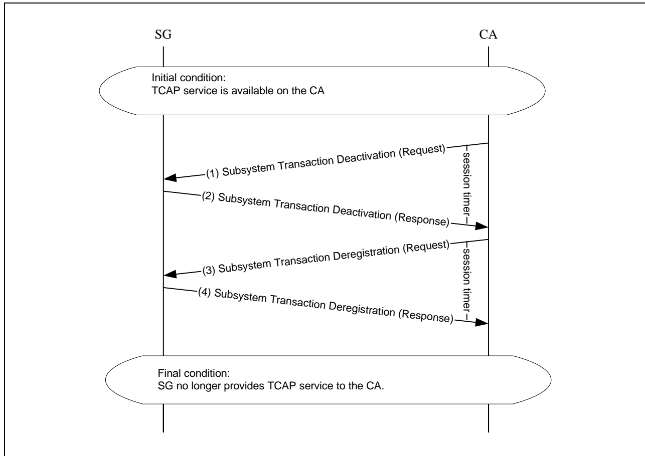
Figure 10. CA Terminates TCAP Service
