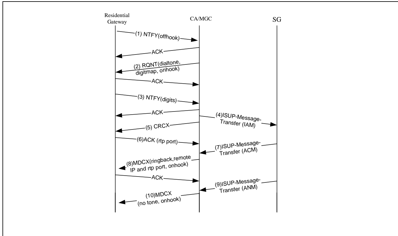
Figure 11. A Typical Origination Communication
