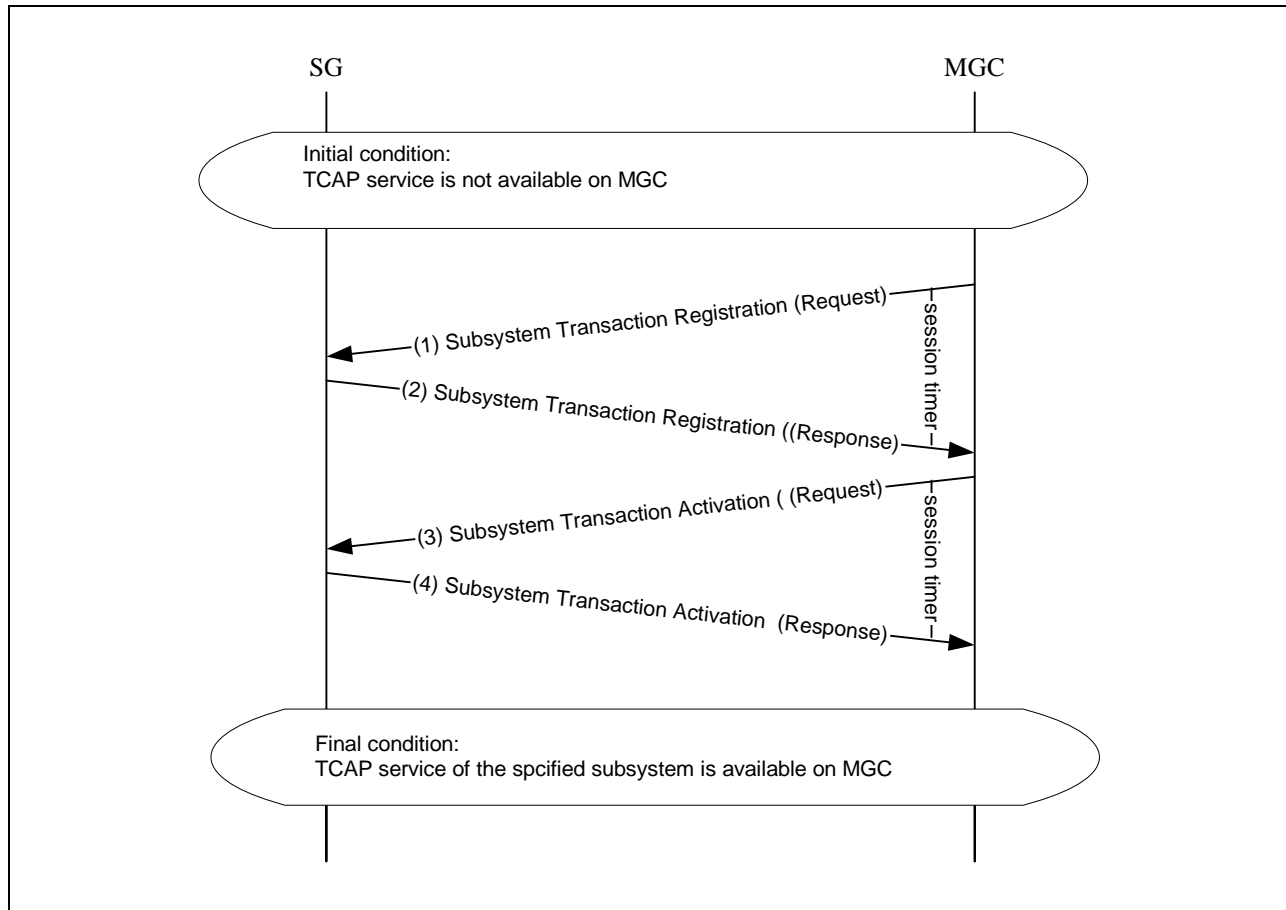
Figure 9. MGC Requests TCAP Service
