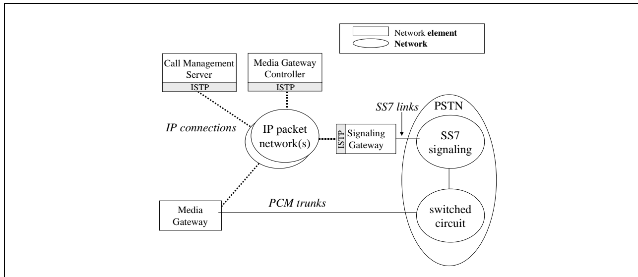
Figure 4. ISTP in Decomposed IPCablecom Gateway
