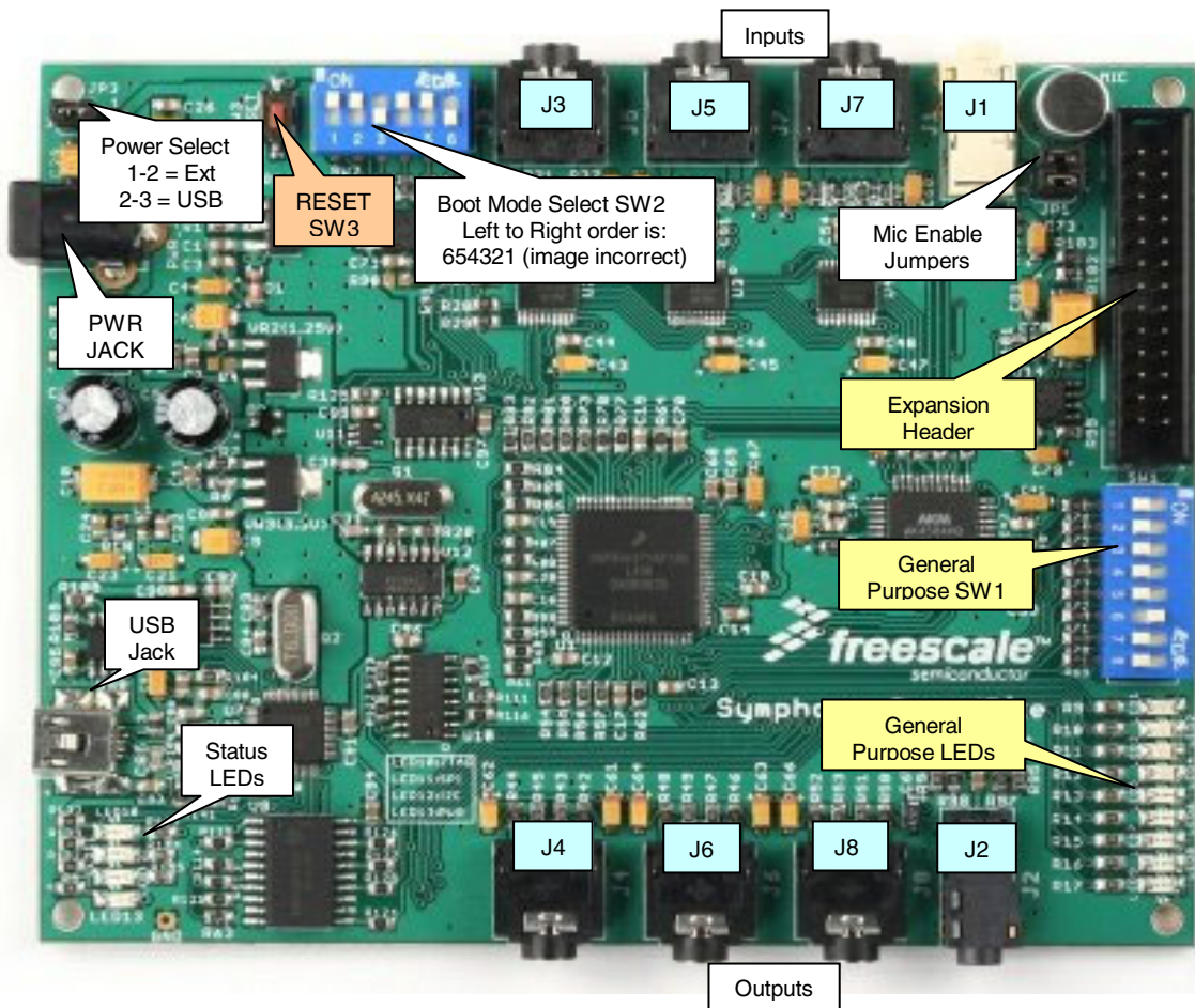
Figure 1-1: Symphony SoundBite Board Layout
