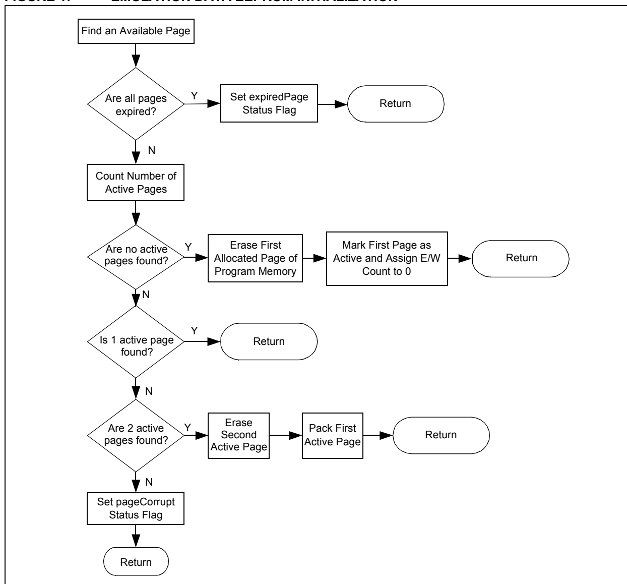
FIGURE 1: EMULATION DATA EEPROM INITIALIZATION
