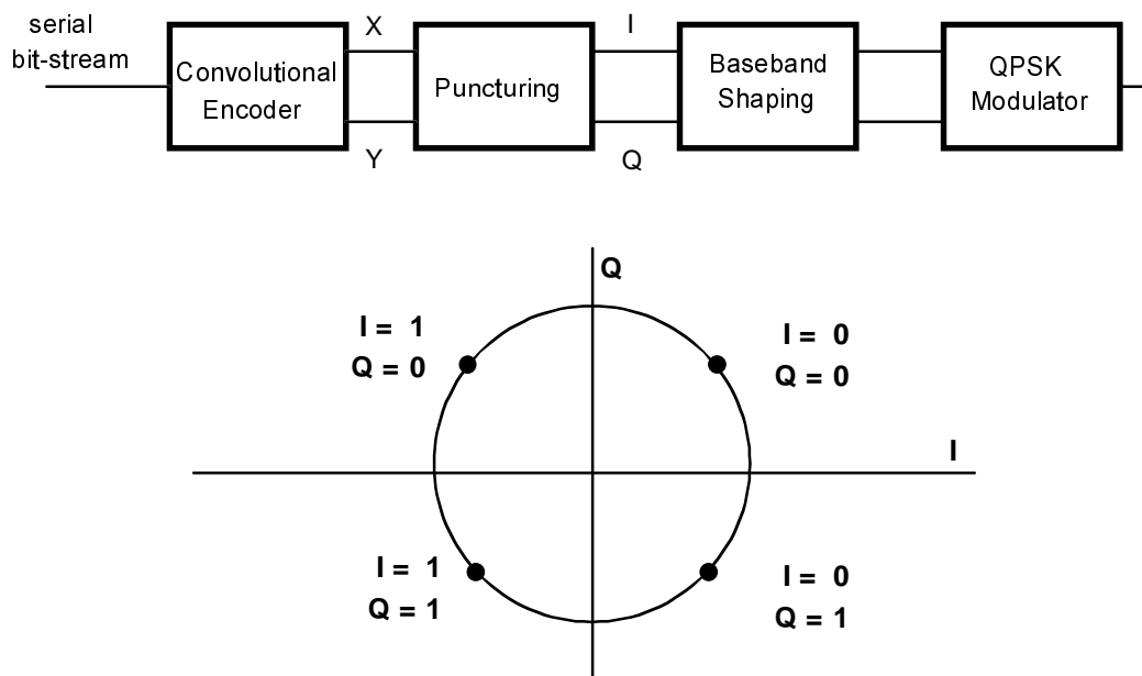
Figure 5: QPSK constellation
